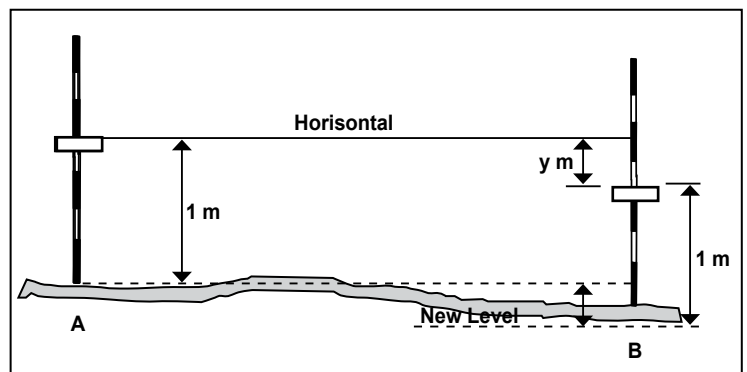
Figure 3-6: Transferring levels
