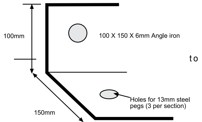
Figure 5-5: Steel Shutter formwork
