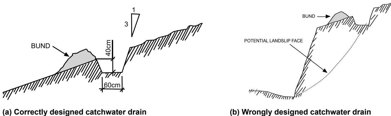
Figure 6-4: Catchwater Drain
