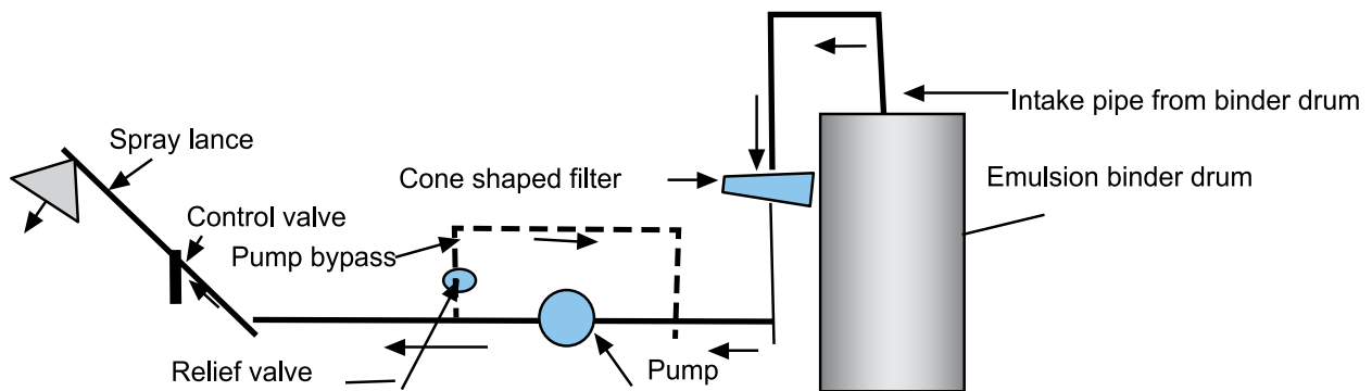
Figure 8-1: Schematic layout of a motorized handsprayer
