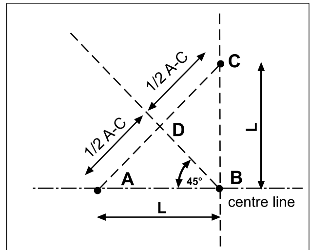
Figure 3-9: Setting out of a 45° angle
