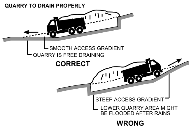
Figure 4-18: Quarry drainage
