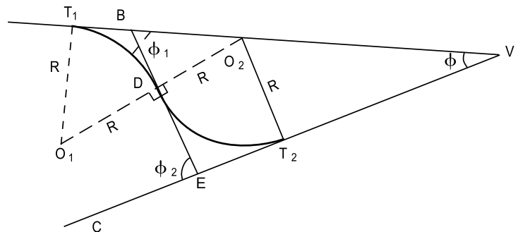
Figure 3-32: Reverse curve with non-parallel straights
