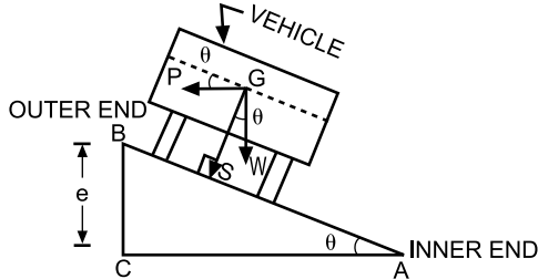
Figure 3-33: Superelevated curve
