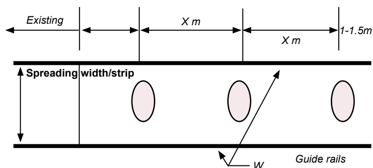
Figure 8-11: Spreading strip
